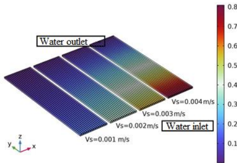
Figure 8: Change of pressure in channels at different speeds, t=13:30 .
