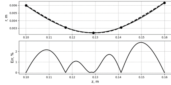
Figure 1: Solving of interpolation task for Example 1.
