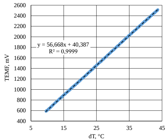
Figure 4: Dependence of the thermoelectromotive force of a thermoelectric converter on the temperature difference dT.
