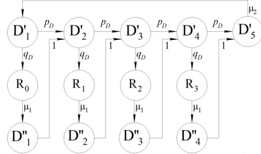
Figure 3: The state-transitions diagram on the degradation cycle for the second type of optical cable repair at n = 5 .
