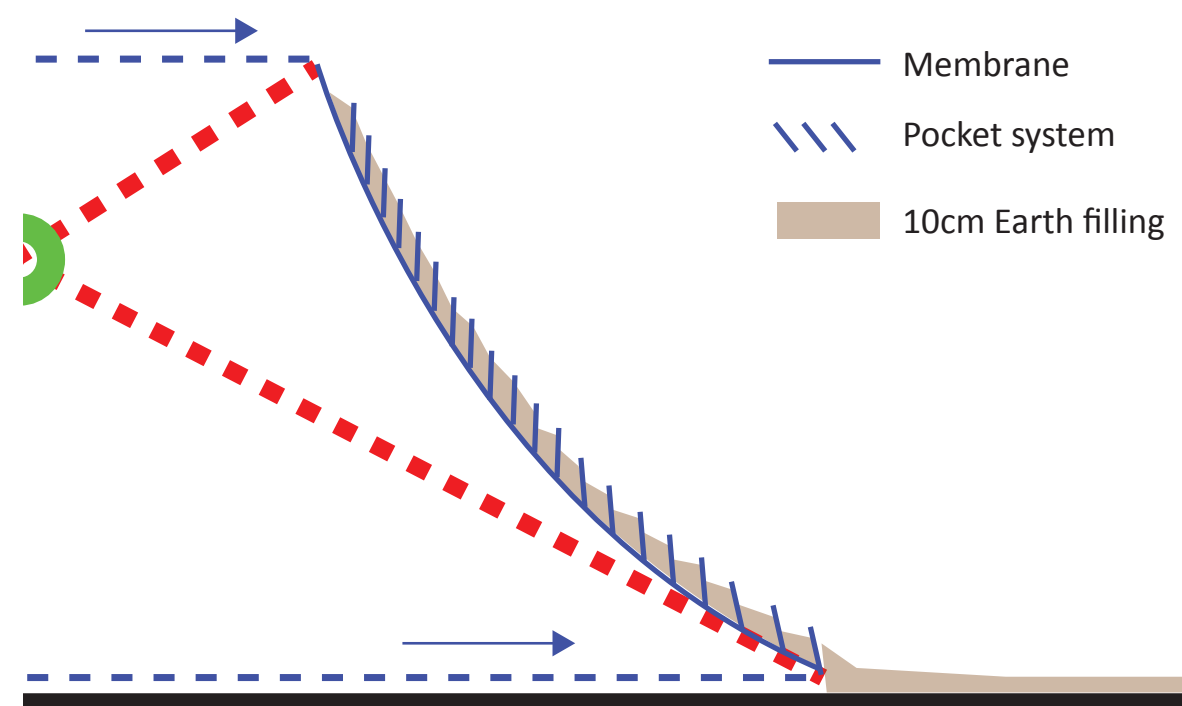
Side Section
