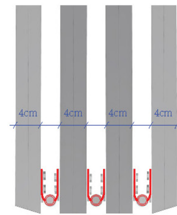
Hinge connection detail : Closed
